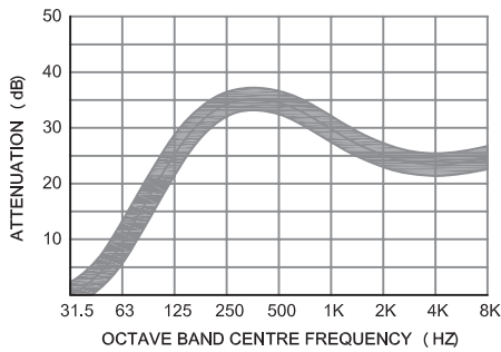
ATTENUATION CURVE
