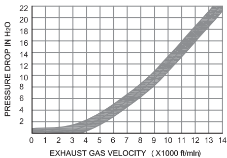
PRESSURE DROP
